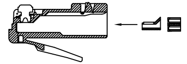
SECTION VIEW WITH NO SHIELD
